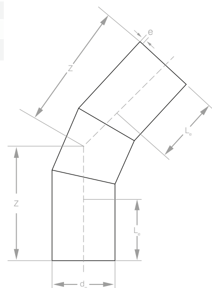
60°/30°/22.5°/11.25° Elbow
