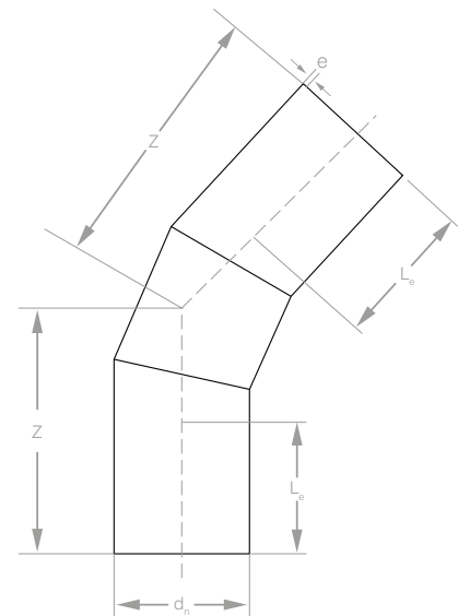
60°/30°/22.5°/11.25° Elbow
