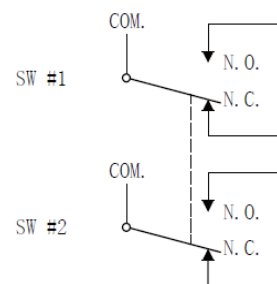
Fig. 6 Closed Position
