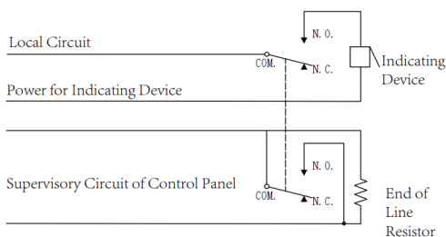
Typical Electrical Connections
