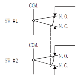
Fig. 7 Open Position
