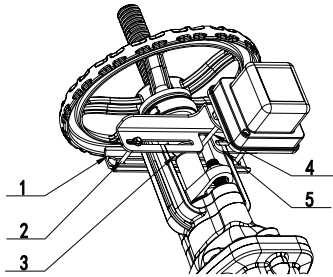
1.Clamp Plate 2.Carriage Rod 3.Groove of Stem 4.Trip Rod 5.Fixing Bracket
